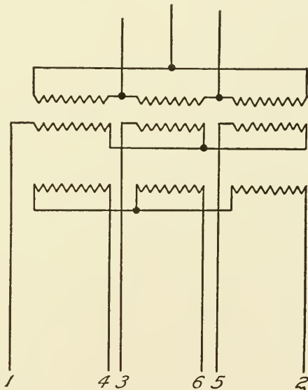
Fig. 34. Six-Phase Y Circuit for Transformer with Two Secondaries
